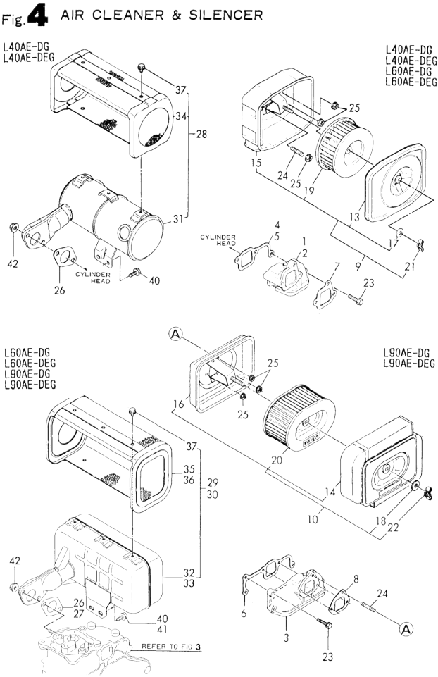
Fig.4. AIR CLEANER & SILENCER
