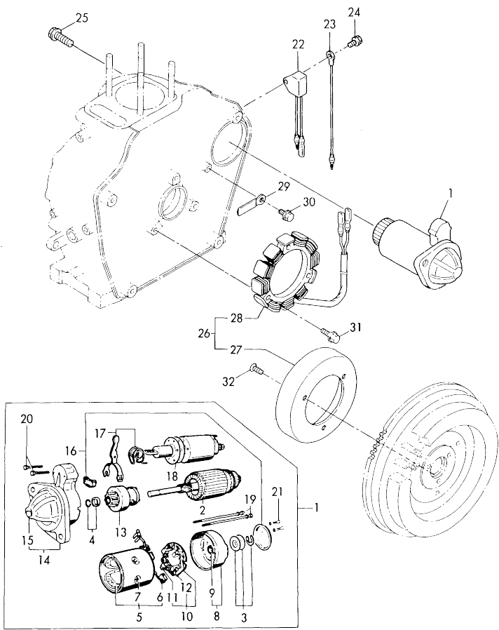
Fig.9 ELECTRIC STARTING DEVICE
