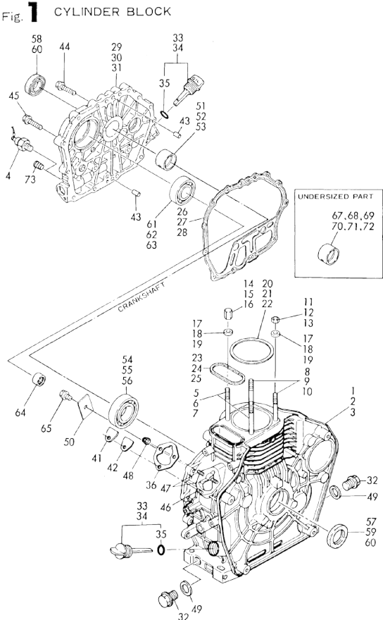
Fig.1. CYLINDER BLOCK
