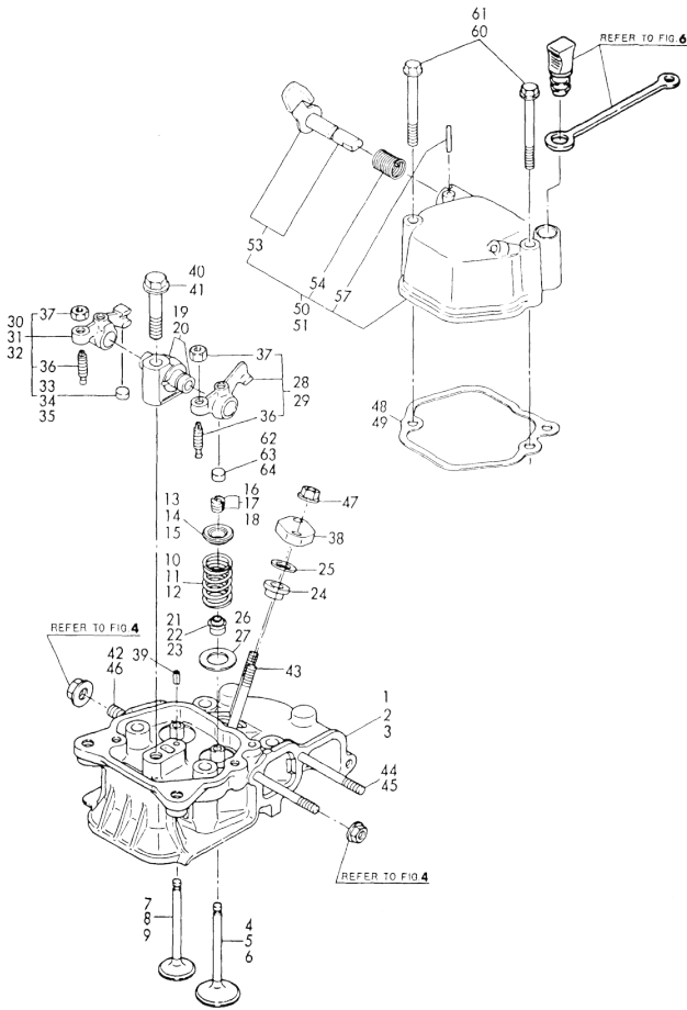
Fig.3 CYLINDER HEAD
