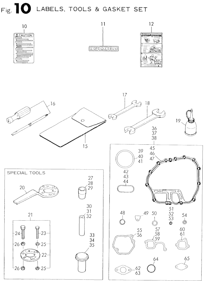
Fig.10. LABEL, TOOL & GASKET SET
