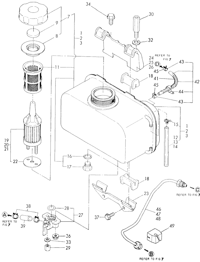
Fig.8 FUEL TANK & PIPE
