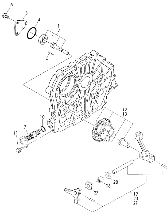
Fig. 5 LUB. OIL & GOVERNOR
