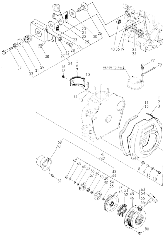
Fig. 6 STARTING & CONTROL
