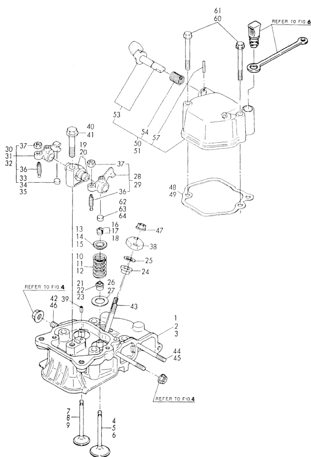
Fig. 3 CYLINDER HEAD
